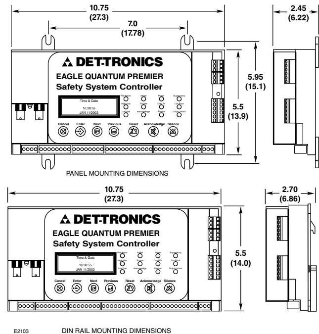
Figure 2—Dimensions of Controller in Inches (Centimeters)
