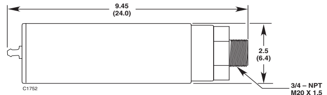
Figure 1—Aluminum PointWatch Unit Dimensions in Inches (cm)
