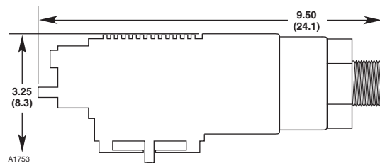
Figure 2—Stainless Steel PointWatch Unit Dimensions in Inches (cm)
