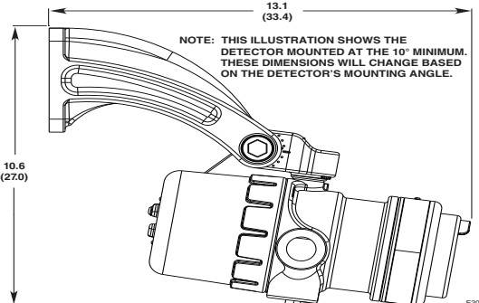
Figure 3—Q9033 Mounting Arm without Collar Attachment Dimensions in Inches (cm) (See Figure 1 for Correct Detector Orientation.)
