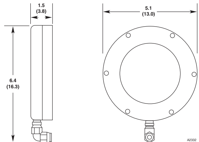
Figure 1—Dimensions of Q1116 in Inches (Centimeters)
