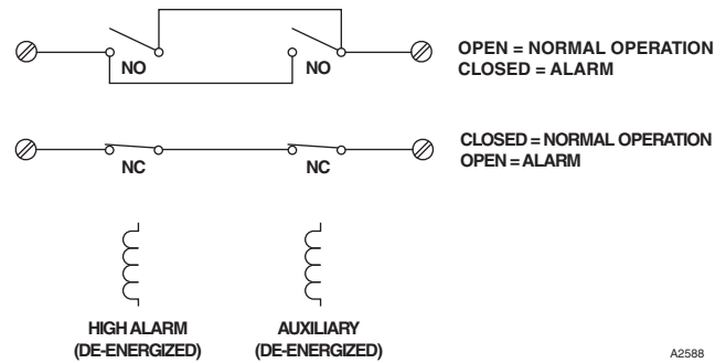
Figure 1—High Alarm and Auxiliary Relays Configured as a De-Energized Pair
