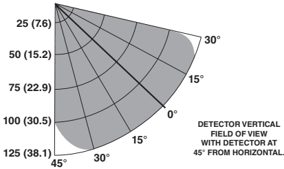
Field of View at Indicated Distance in Feet (m) for Hydrogen at Very High Sensitivity (30 inch plume, with 100 SLPM flow rate)
