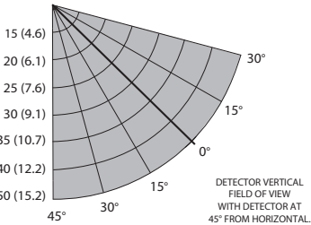
Field of View at Indicated Distance in Feet (m) for Syngas at Medium Sensitivity (30 inch plume, with 120 SLPM flow rate)
