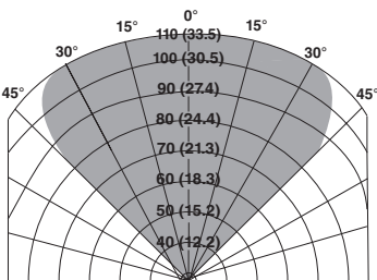
Field of View at Indicated Distance in Feet (m) for Hydrogen at Very High Sensitivity (30 inch plume, with 100 SLPM flow rate)
