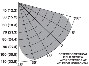
Field of View at Indicated Distance in Feet (m) for Syngas at Very High Sensitivity (30 inch plume, with 120 SLPM flow rate)
