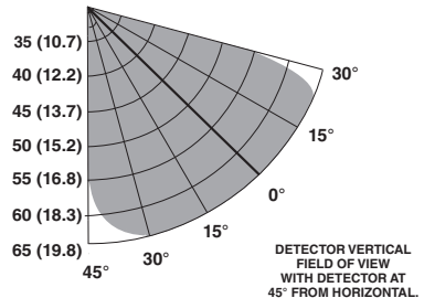
Field of View at Indicated Distance in Feet (m) for Methane at Very High Sensitivity (30 inch plume, with 40 SLPM flow rate)
