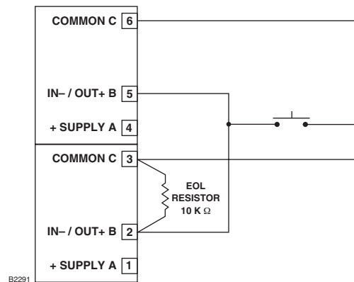
Figure 5—Supervised Input Configuration – Class A
