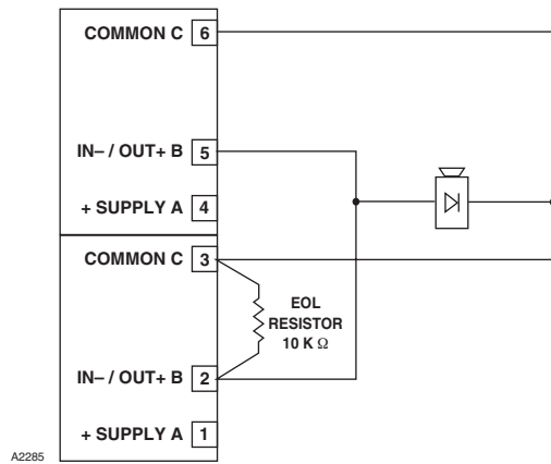
Figure 12—Supervised Output Configuration (Notification)— Class A
