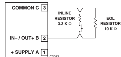
Figure 6—Supervised Input Configuration (Opens and Shorts) – Class B
