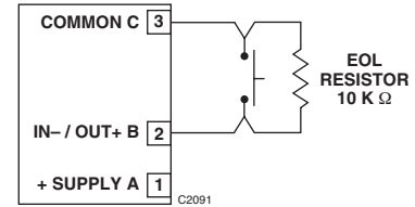
Figure 4—Supervised Input Configuration – Class B
