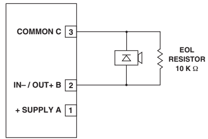
Figure 11—Supervised Output Configuration (Notification)— Class B
