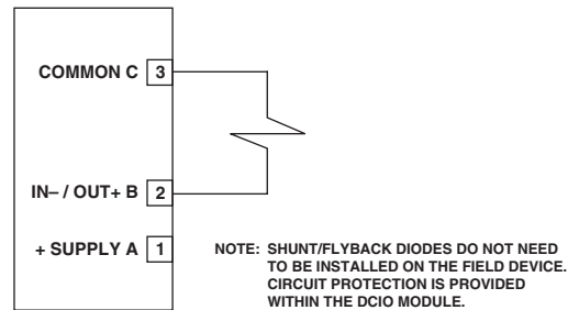
Figure 13—Supervised Output Configuration (Agent Release)
