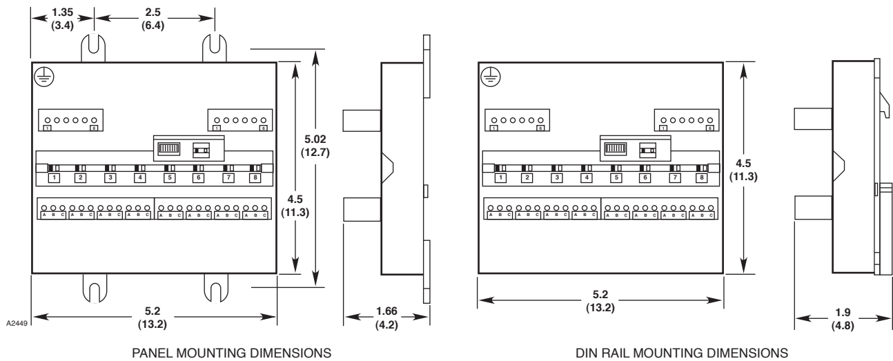
Figure 1—Dimensions of the EDIO Module in Inches (Centimeters)
