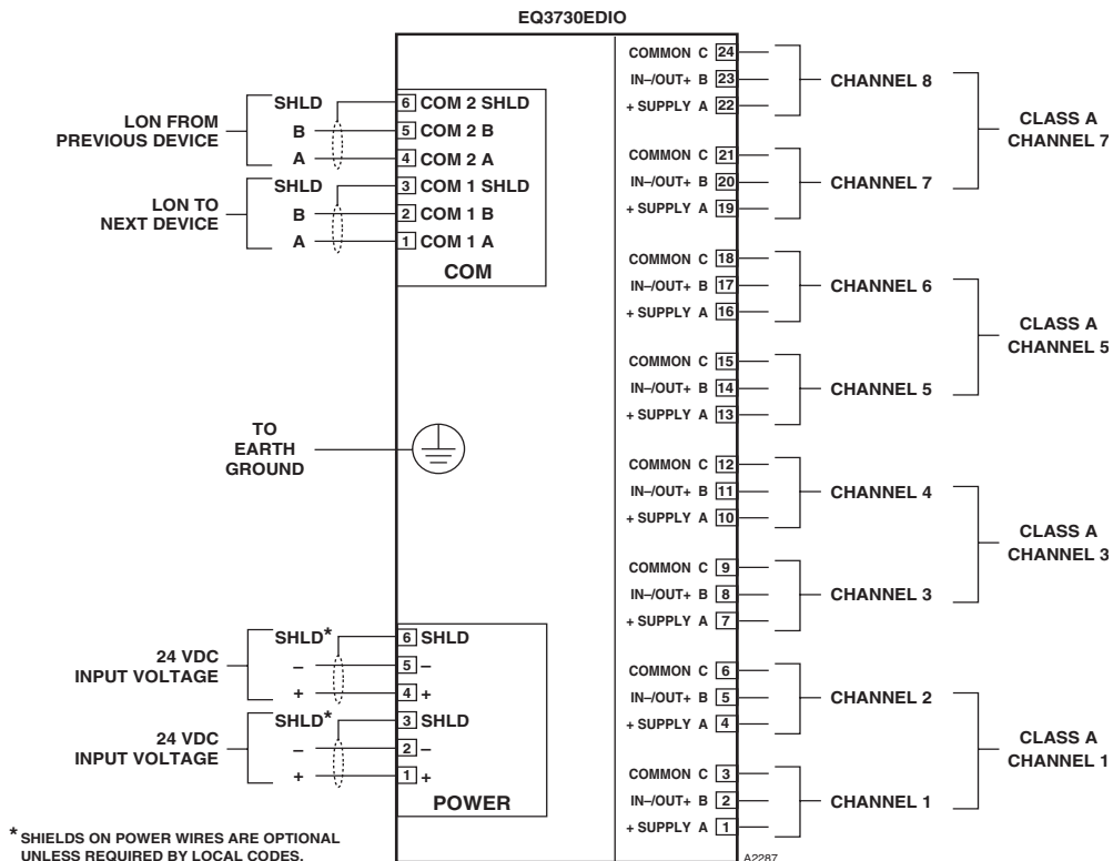
Figure 2—EDIO Module Wiring Terminals
