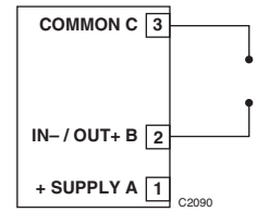
Figure 3—Unsupervised Input Configuration
