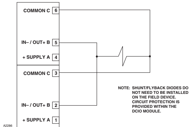
Figure 14—Supervised Output Configuration (Agent Release)— Class A Wiring
