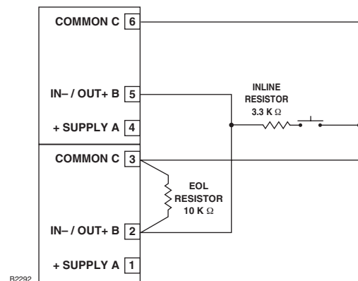
Figure 7—Supervised Input Configuration (Opens and Shorts) – Class A
